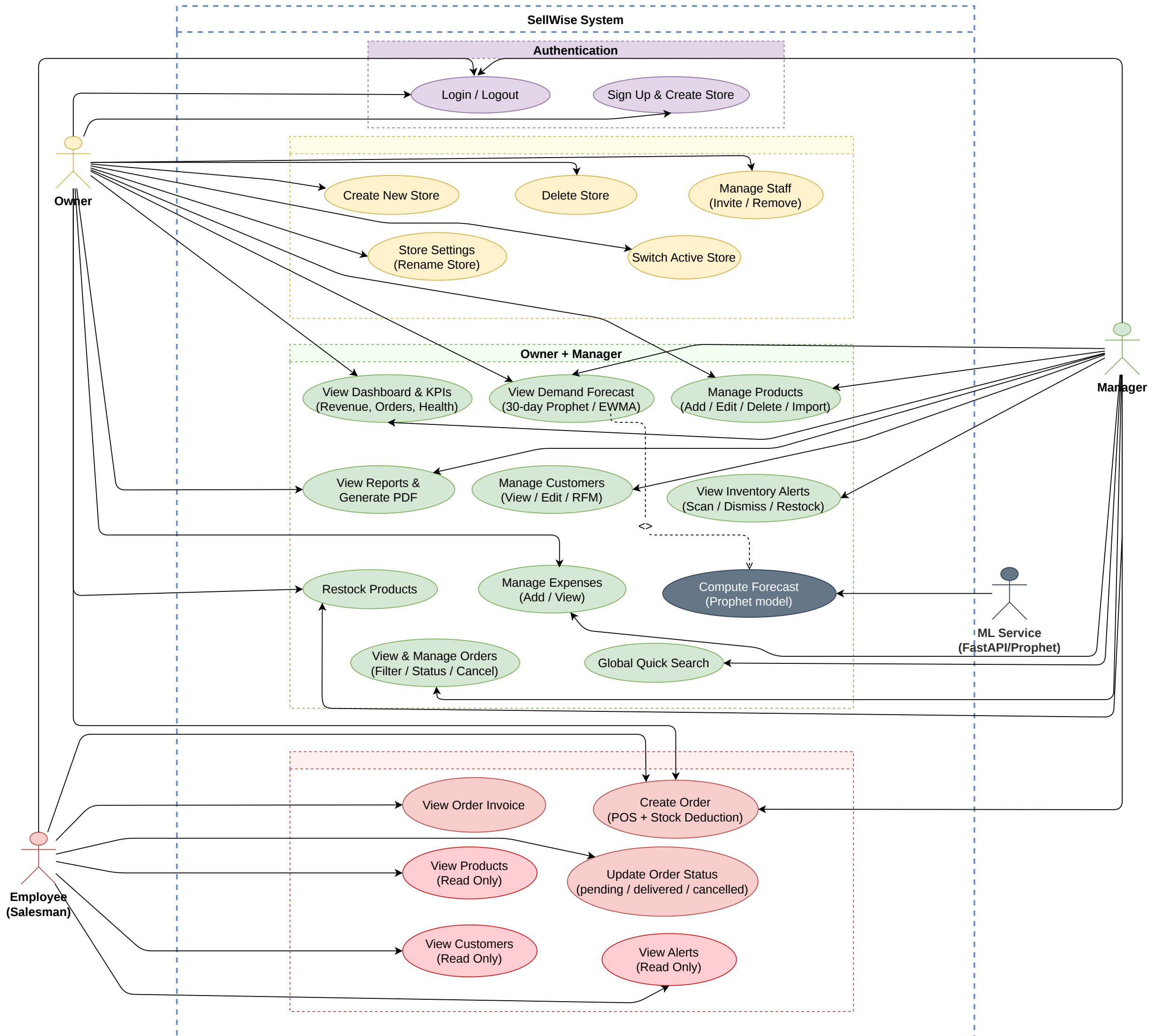
SellWise — Role-Based Use Case Diagram
